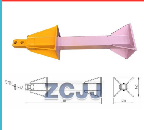
Fixing Angle for Zoomlion 7030
