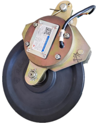
Load Limiter 8t
